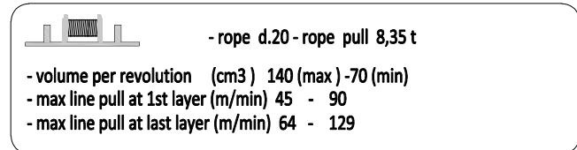
Double winch
