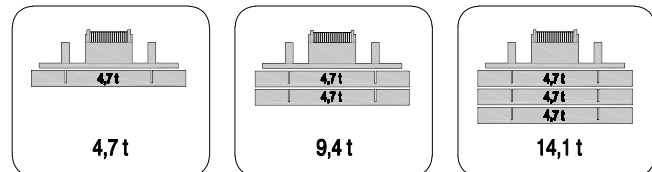
Divisible counterweight with automatic unloading
