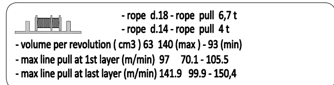
Double winch
