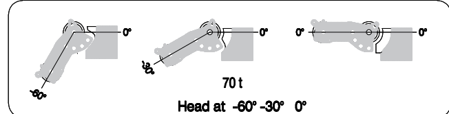
Primary winch
