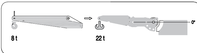
0,5 meters hook for reclinable boom head at -60° -30° 0°
